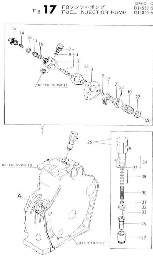
Fig.17. FUEL INJECTION PUMP
