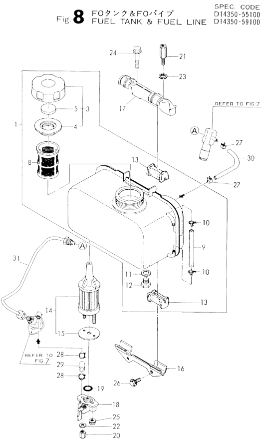
Fig.8. FUEL TANK & FUEL PIPE
