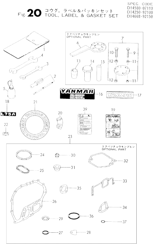
Fig.20. LABEL,TOOL & GASKET SET
