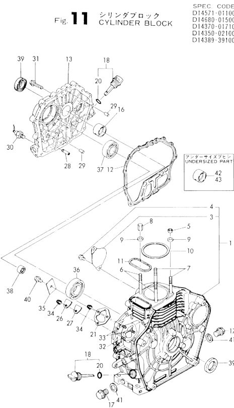
Fig.11. CYLINDER BLOCK
