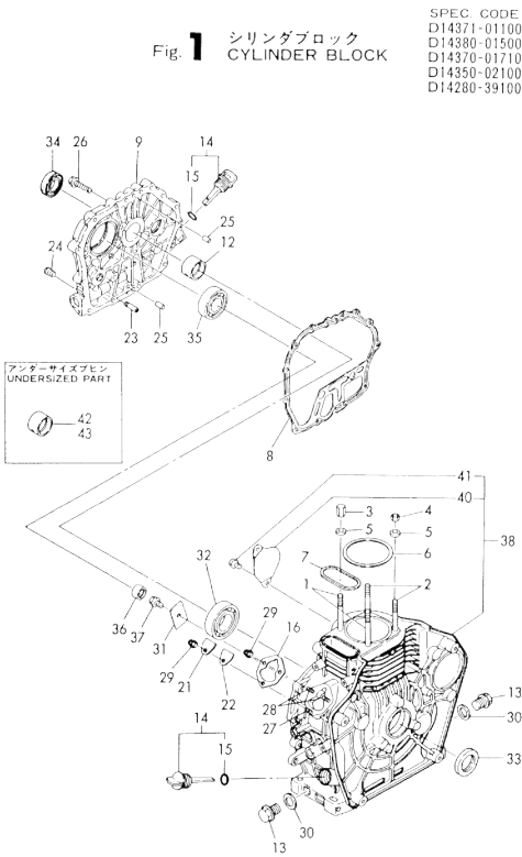
Fig.1. CYLINDER BLOCK
