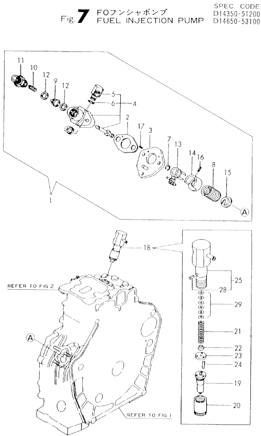
Fig.7. FUEL INJECTION PUMP
