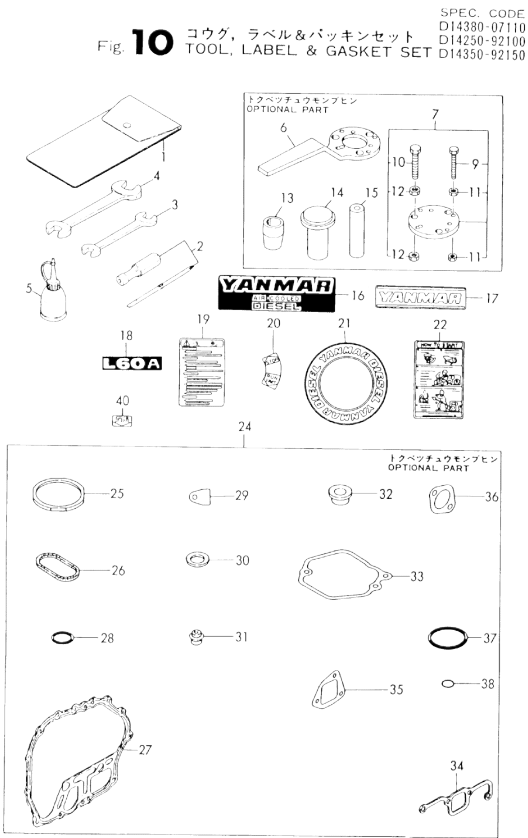
Fig.10. TOOL,LABEL & GASKET SET
