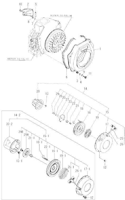
Fig.16. COOLING & STARTING DEVICE
