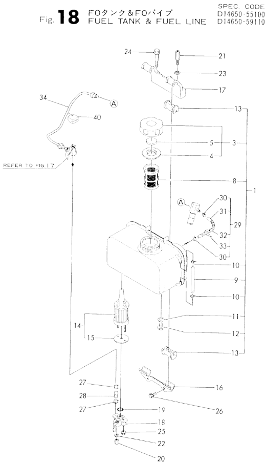
Fig.18. FUEL TANK & FUEL PIPE
