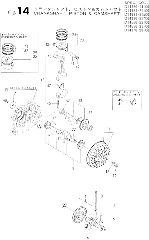
Fig.14. CRANKSHAFT,PISTON & CAMSHAFT
