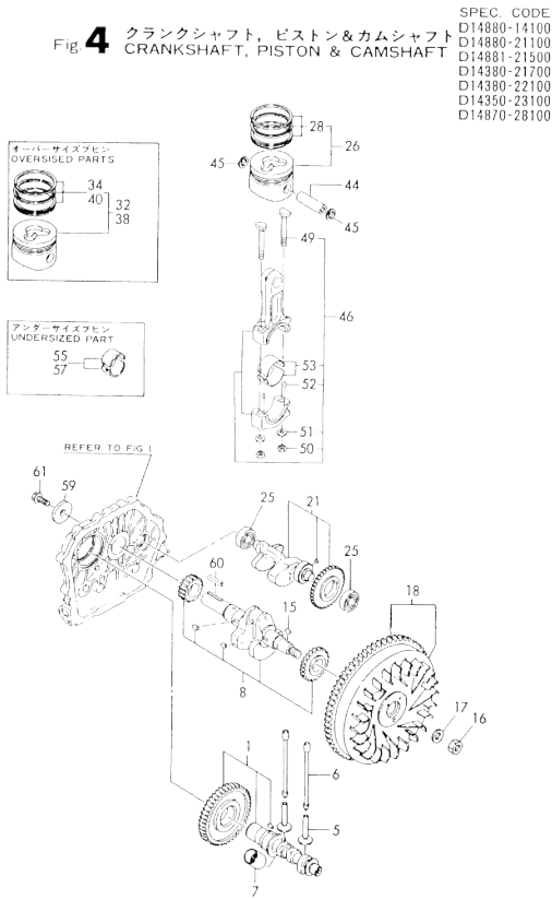
Fig.4. CRANKSHAFT,PISTON & CAMSHAFT
