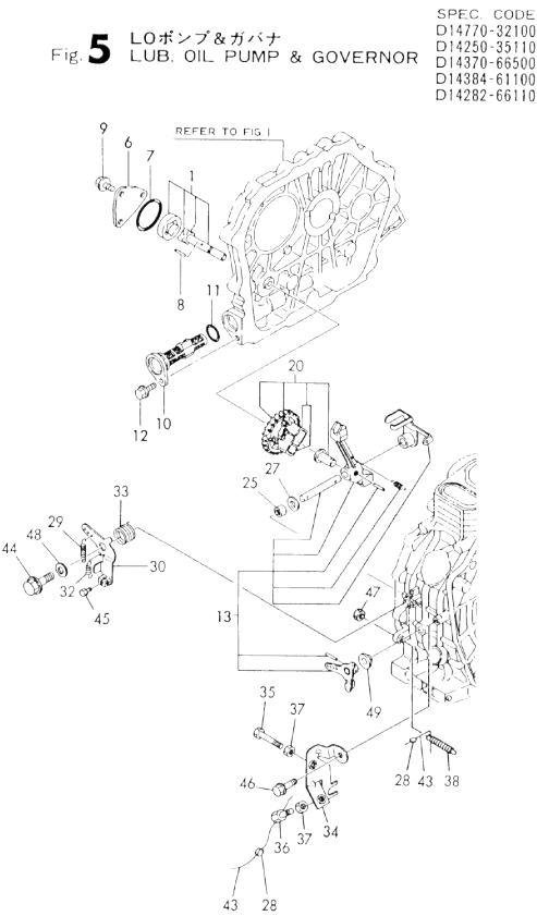
Fig.5. LUB. OIL PUMP & GOVERNOR
